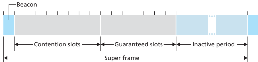
Figure 6.17 ♦ Zigbee 802.14.4 super-frame structure
