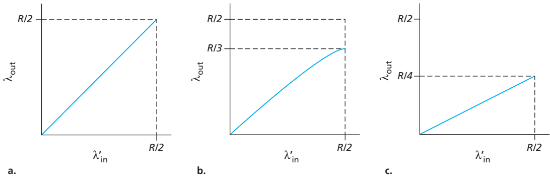
Figure 3.46 ♦ Scenario 2 performance with finite buffers
